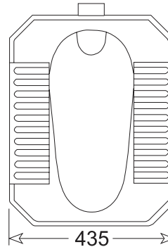
HD13 | Squatting Pan Without Trap Size: 585 x 435 x 300mm
