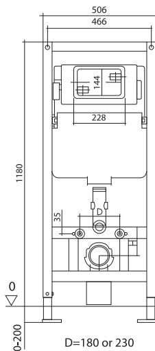
HDG30041 | Concealed Cistern With B20 Push Button With Frame
