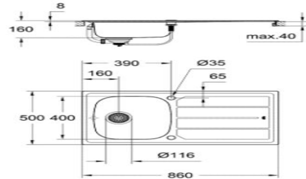
SPECIFICATION SINGLE BOWEL 31552SD0
