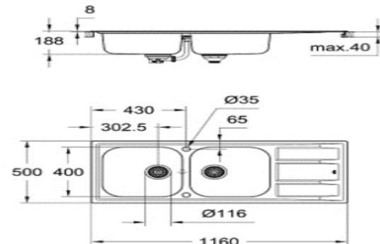
SPECIFICATION DOUBLE BOWEL 31587SD0
